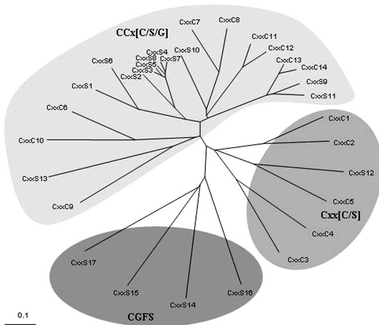
Figure 2. Phylogenetic tree of the various A. thaliana Grx isoforms. This tree was drawn using ClustalW. The protein entry codes are identical to those of table 1 and figure 1. Three classes can be distinguished according essentially to the active site sequences: CGFS, Cxx[C/S] and CCx[C/S/G].
